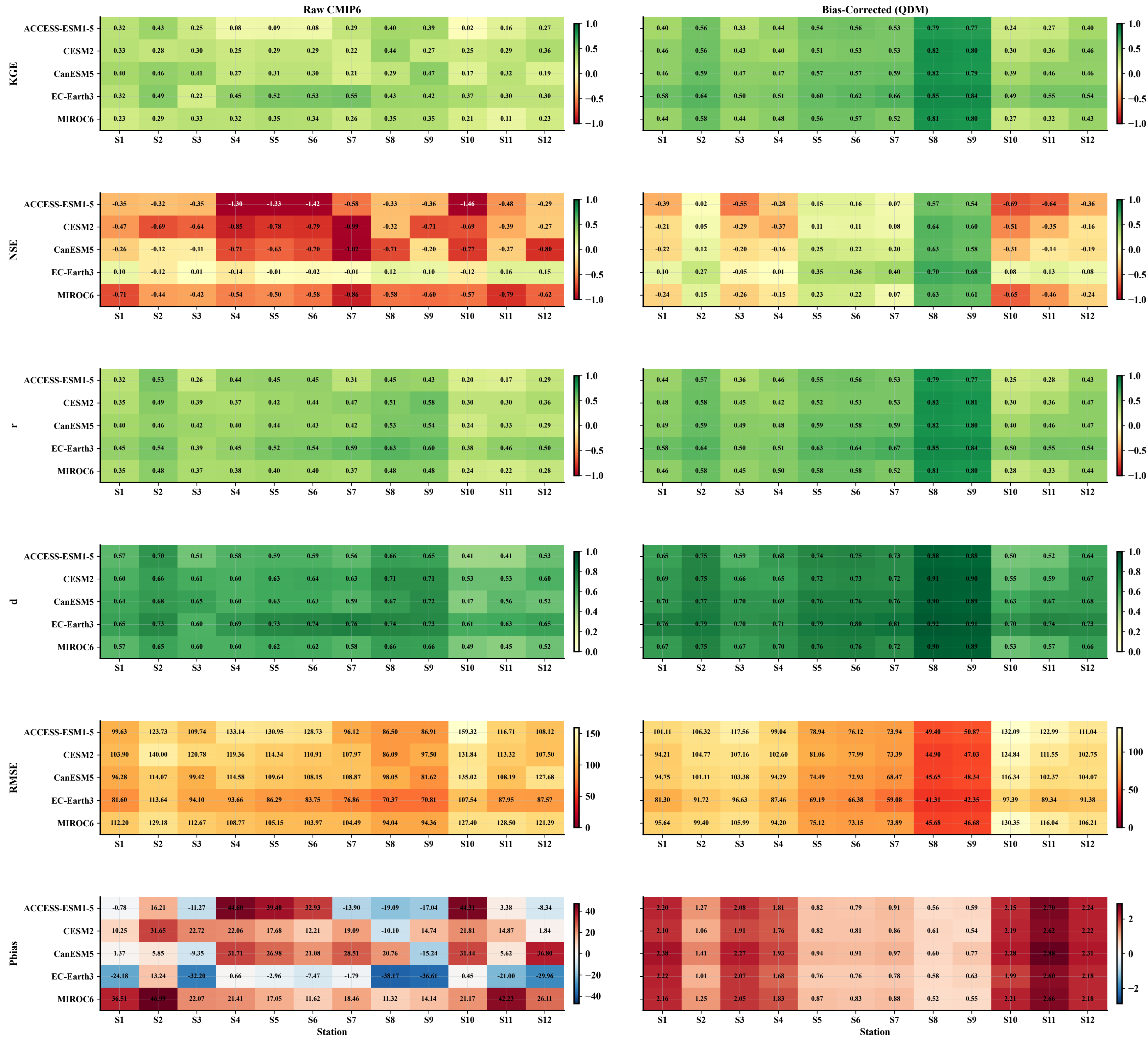
Model Performance Heatmap - Monthly Scale Raw CMIP6 (left) vs Bias-Corrected QDM (right) | Obs: 1981-2014
